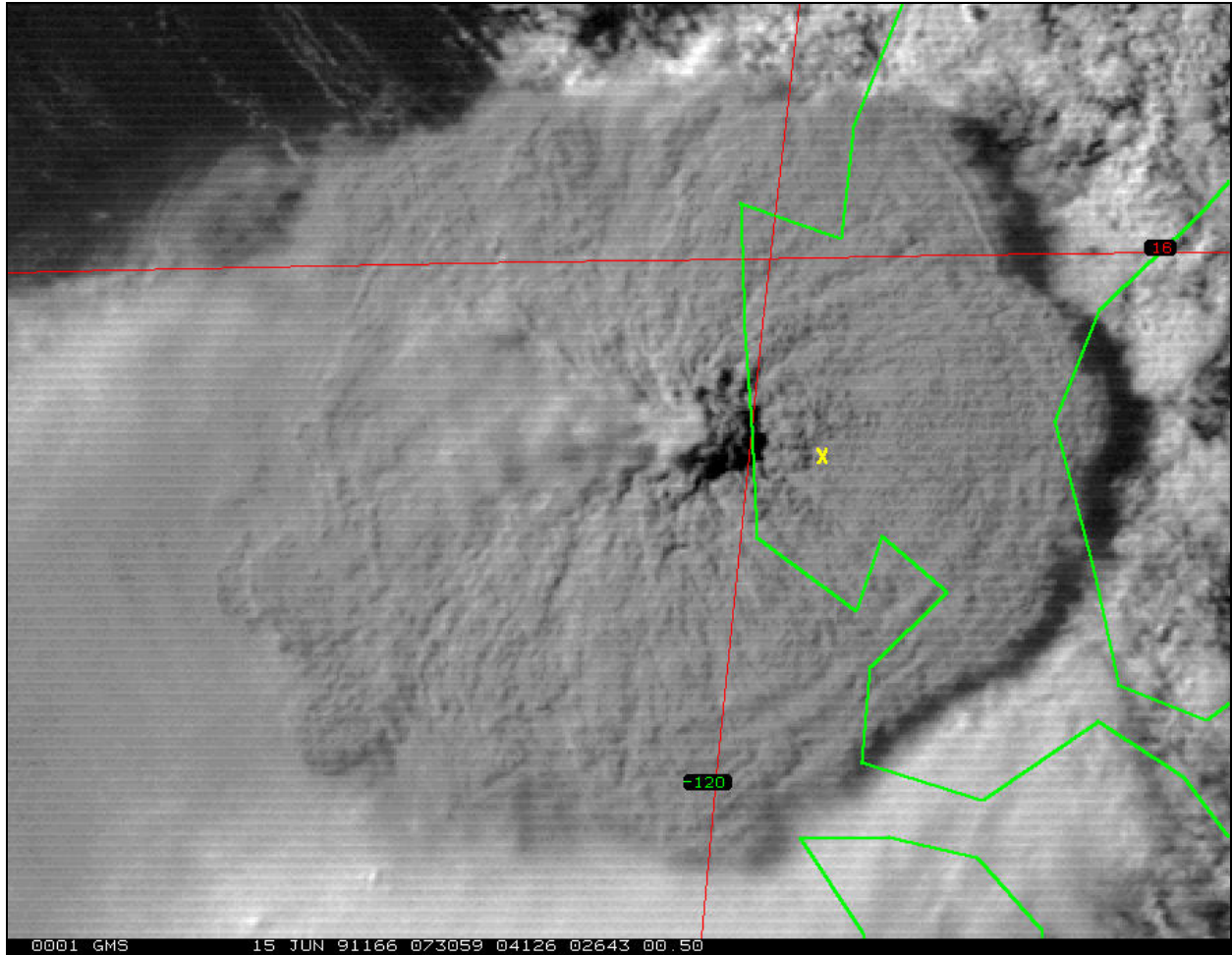
Figure 1 Example of a satellite image of an enormous volcanic plume. This image was acquired by the Japanese GMS satellite in the visible part of the spectrum. The plume is from the June 1991 eruption of Pinatubo in the Philippines. At the time this image was acquired, the plume covered an area several hundred thousand square kilometers.
