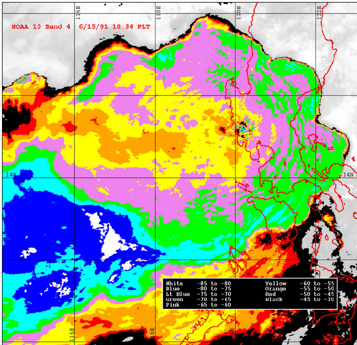
Figure 9 Example of a temperature map for the Pinatubo eruption plume. The temperatures in this image were derived from AVHRR channel 4 data.
